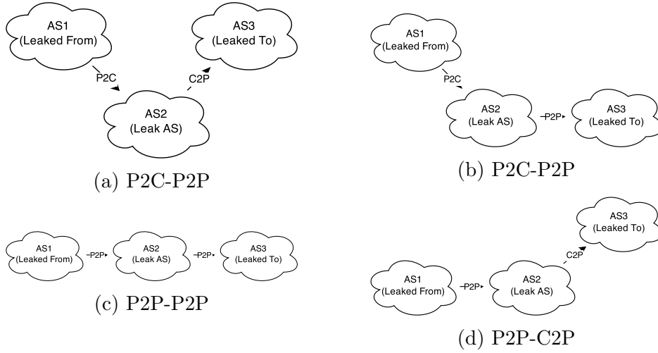
Figure 3.4: Violation types
