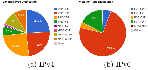
Figure 5.4: Violation types per IP version
